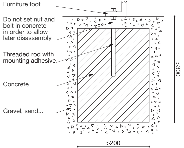
With foundation with ground anchor
